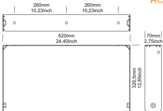
XL-UH12 Wall metal bracket to mount in horizontal position
