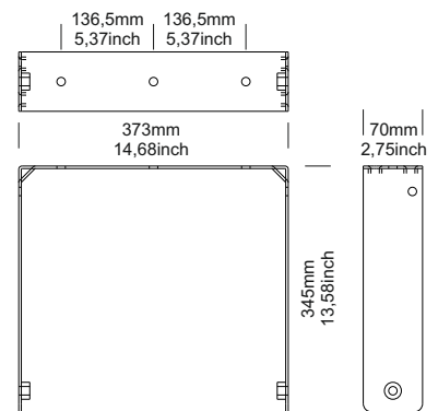
XL-UV12 Wall metal bracket to mount in vertical position
